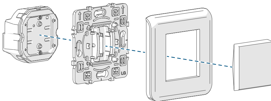
Homematic IP Shading Actuator for brand switches
