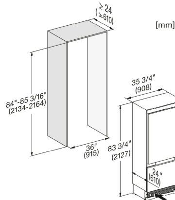
KF2902Vi, KF2912Vi, KF2901Vi, KF2911Vi, Installation, MasterCool, Skizze
