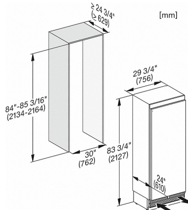
K2801Vi, K2811Vi, K2802Vi, K2812Vi, Innenraum, MasterCool, Skizze
