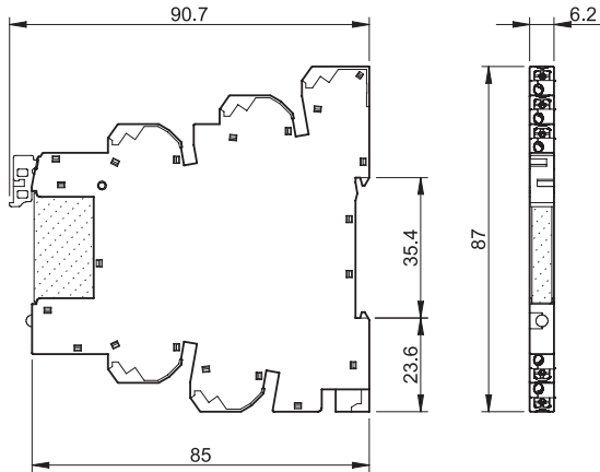
Typ 39.70 39.71 Push-In - Klemmen
