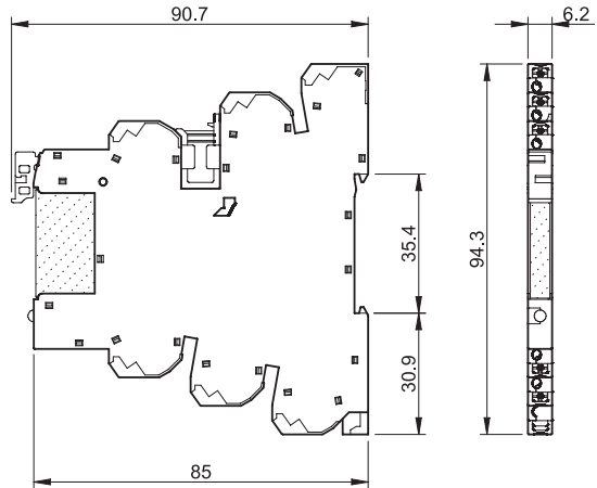
Typ 39.90 39.91 Push-In - Klemmen
