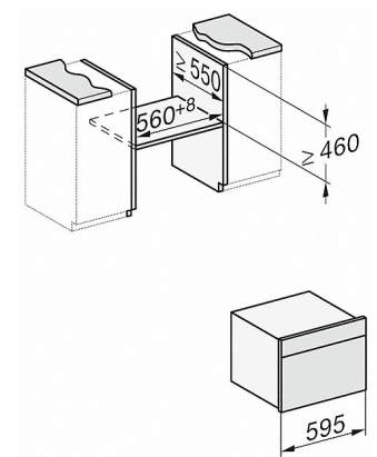
H7x4xBM, Skizze
