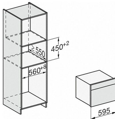
H7x40BM/BMX, Skizze
