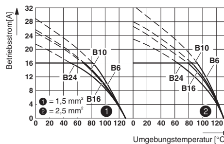
Derating-Diagramm
