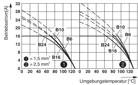
Derating-Diagramm
